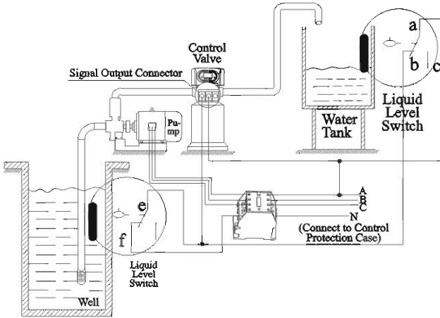
Figure11 Wiring of Liquid Level Switch in Water Tank Controls Inlet Pump
