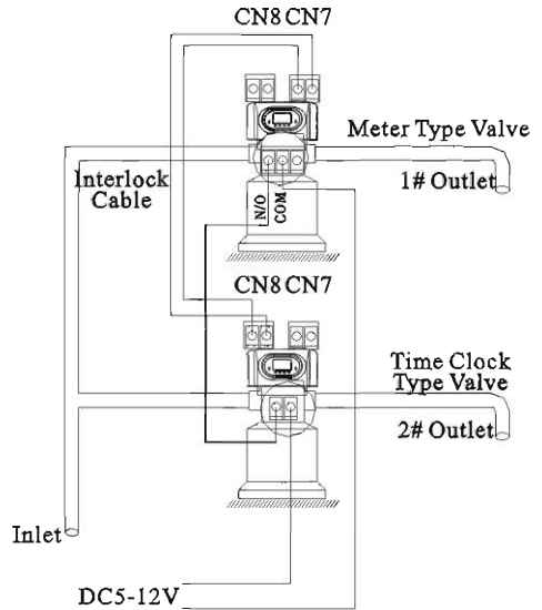
Figure18 All in service, regenerate sequence
